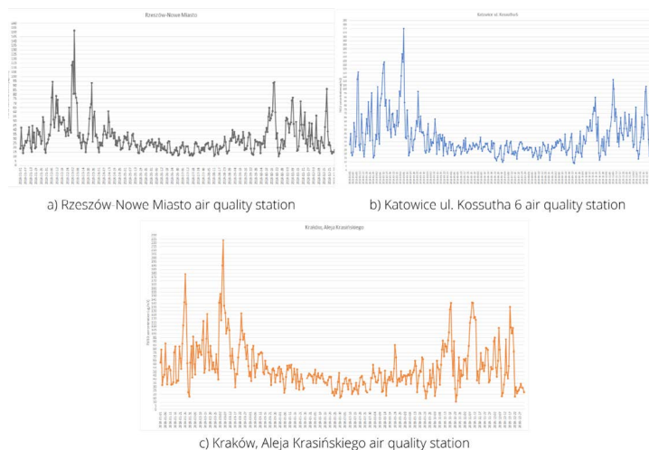
Figure 4. 2018 daily average concentration PM10 in Rzeszów, Katowice, and Kraków air quality stations
