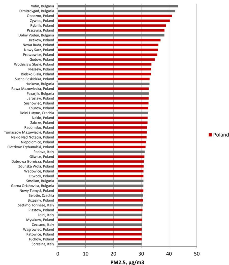
Figure 1. 50 most polluted cities in the European Union in 2018 [3]
