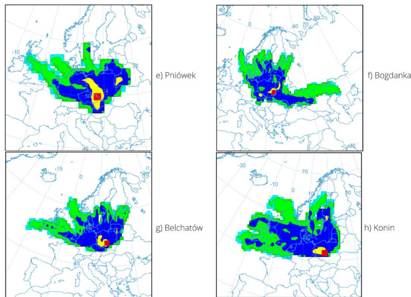
Figure 6. Trajectory frequency analysis of 168H of forward trajectory of PM10 particles from different coal mine sites
