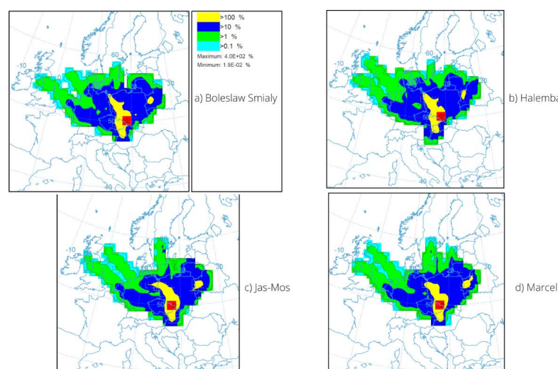
Figure 5. Trajectory frequency analysis of 168H of forward trajectory of PM10 particles from different coal mine sites
