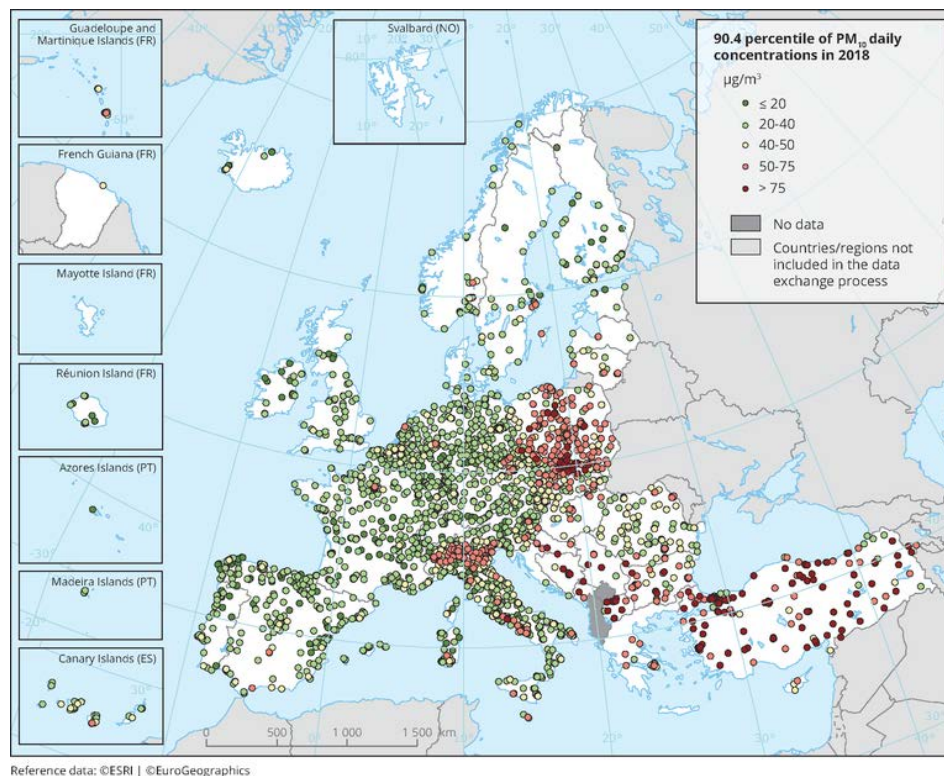
Figure 2. Map of 90.4 percentile of PM10 daily concentrations in 2018 [7]
