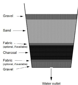
Figure 1: Optimised layering of charcoal – sand – filter
